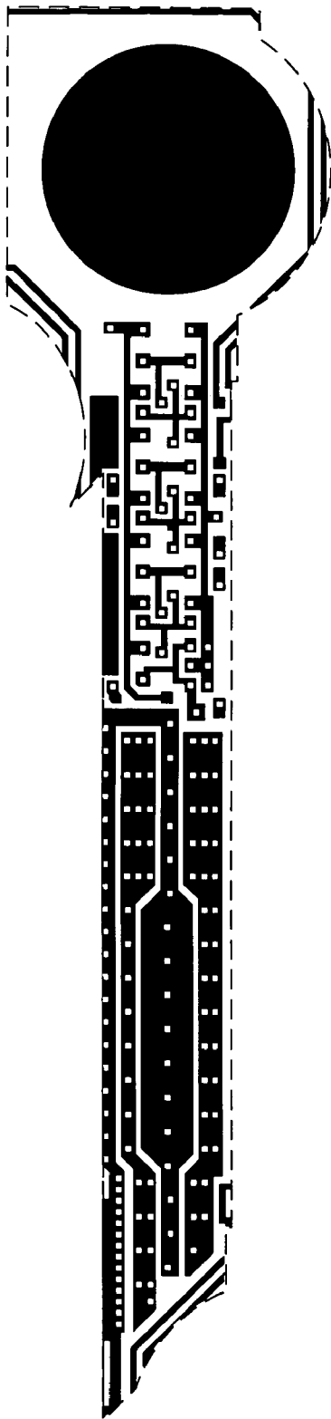
Metal 1 mask
